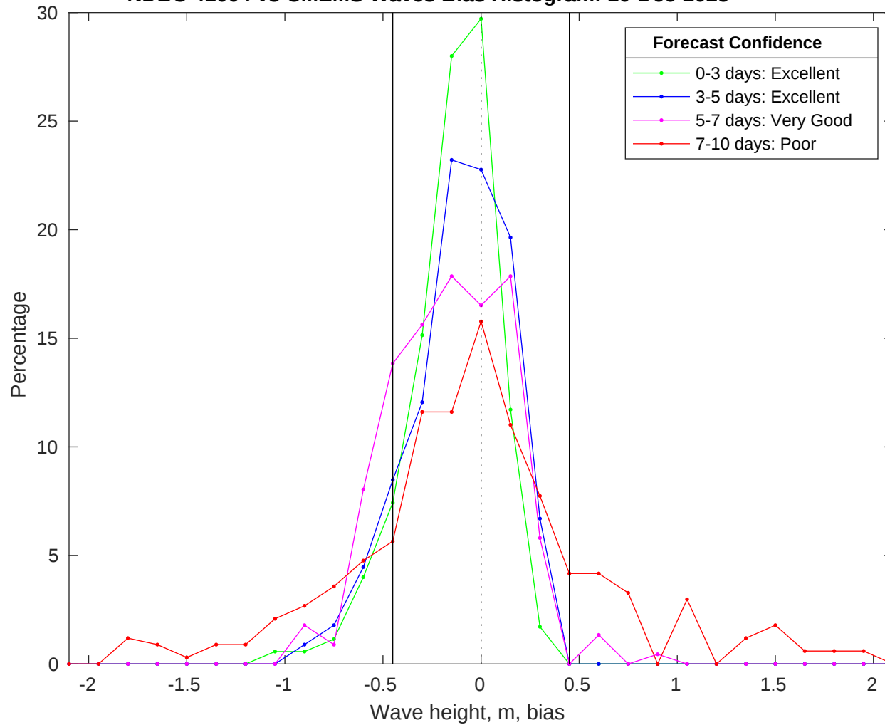
NDBC 41004 vs CMEMS Waves Bias Histogram: 10-Dec-2025
