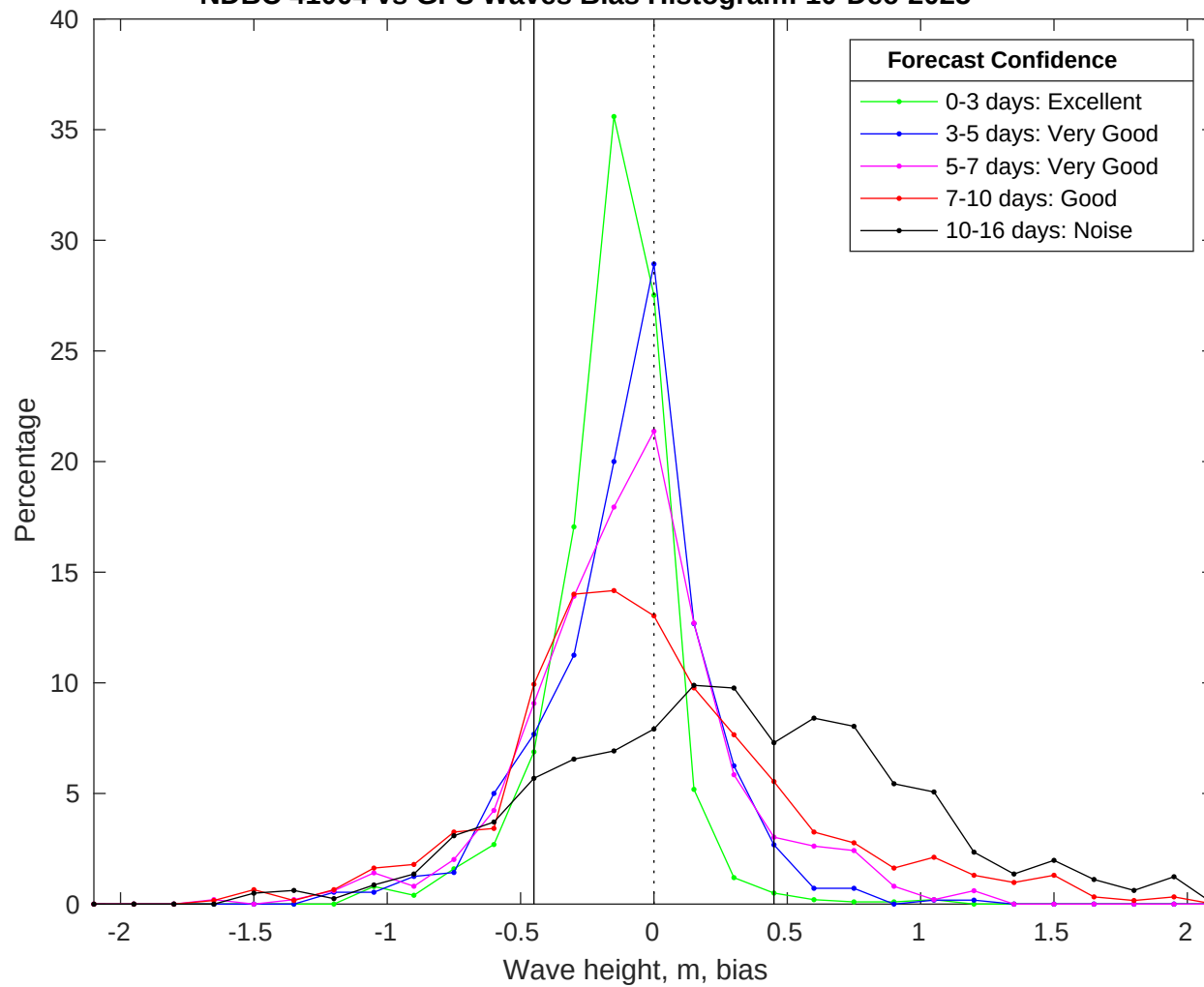
NDBC 41004 vs GFS Waves Bias Histogram: 10-Dec-2025
