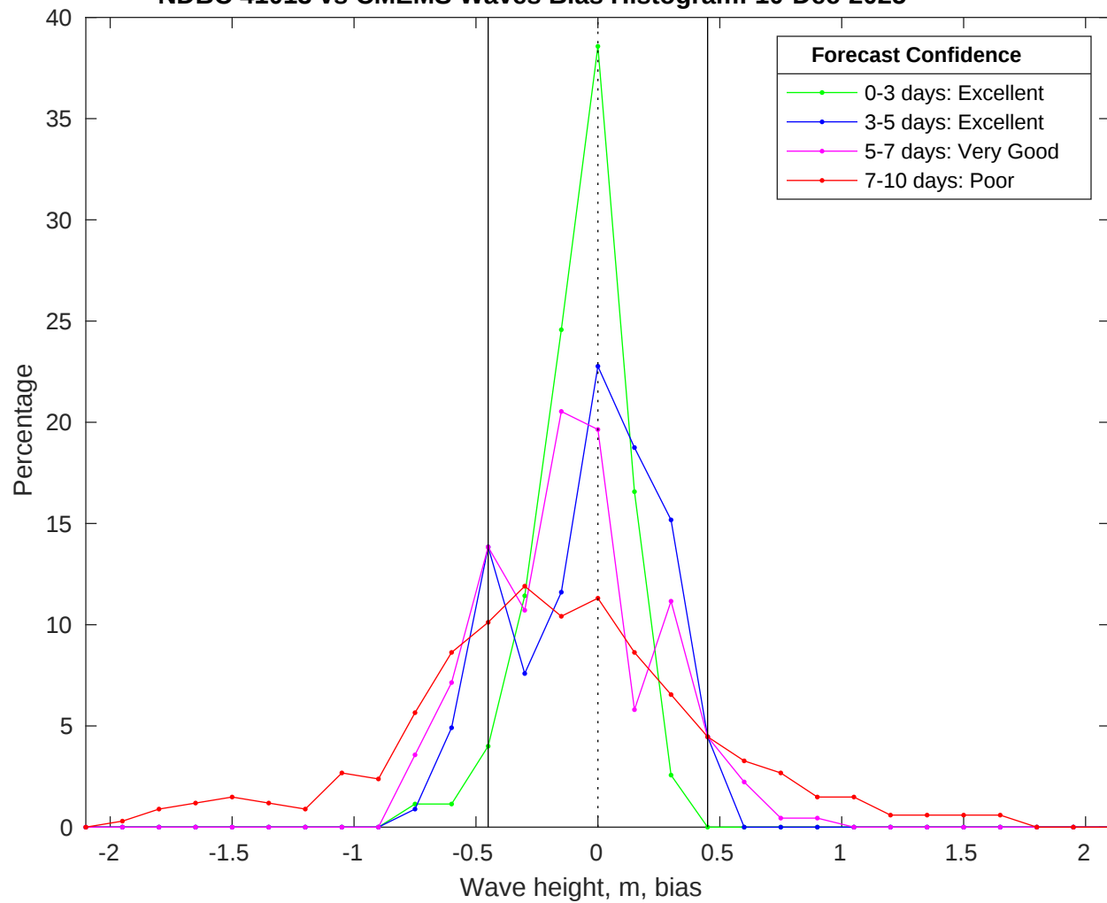
NDBC 41013 vs CMEMS Waves Bias Histogram: 10-Dec-2025
