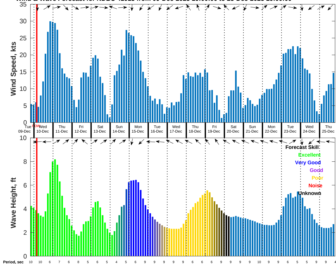
Wind & Wave Forecast for NDBC 41013 from 09-Dec-2025 19:00:00 to 25-Dec-2025 19:00:00
