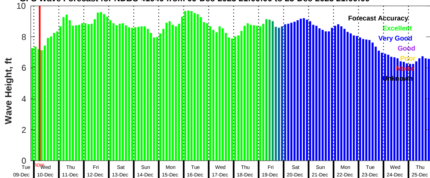
GFS Wave Forecast for NDBC 41040 from 09-Dec-2025 21:00:00 to 25-Dec-2025 21:00:00
