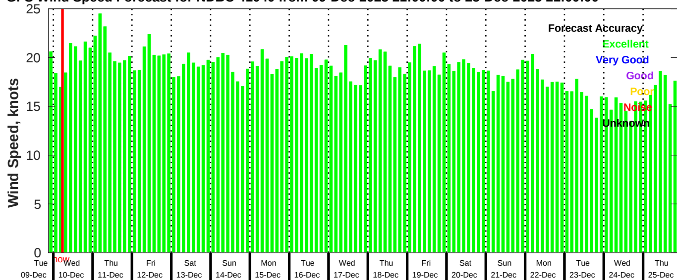
GFS Wind Speed Forecast for NDBC 41040 from 09-Dec-2025 21:00:00 to 25-Dec-2025 21:00:00
