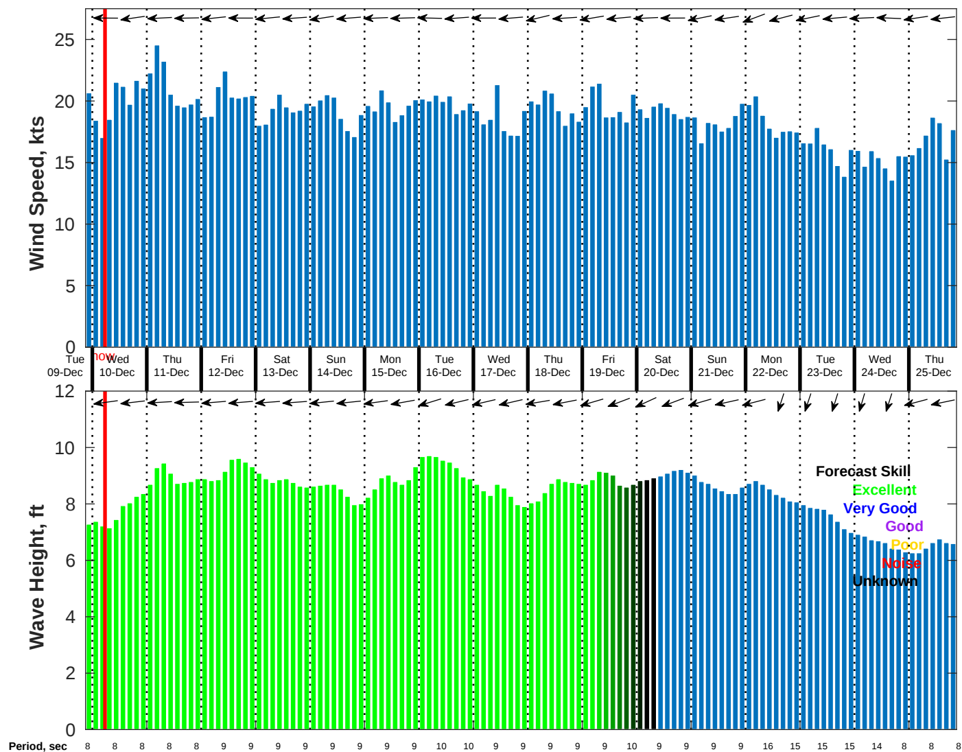
Wind & Wave Forecast for NDBC 41040 from 09-Dec-2025 21:00:00 to 25-Dec-2025 21:00:00
