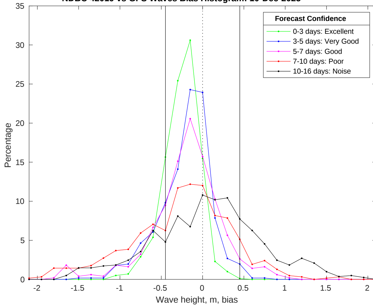
NDBC 42019 vs GFS Waves Bias Histogram: 10-Dec-2025
