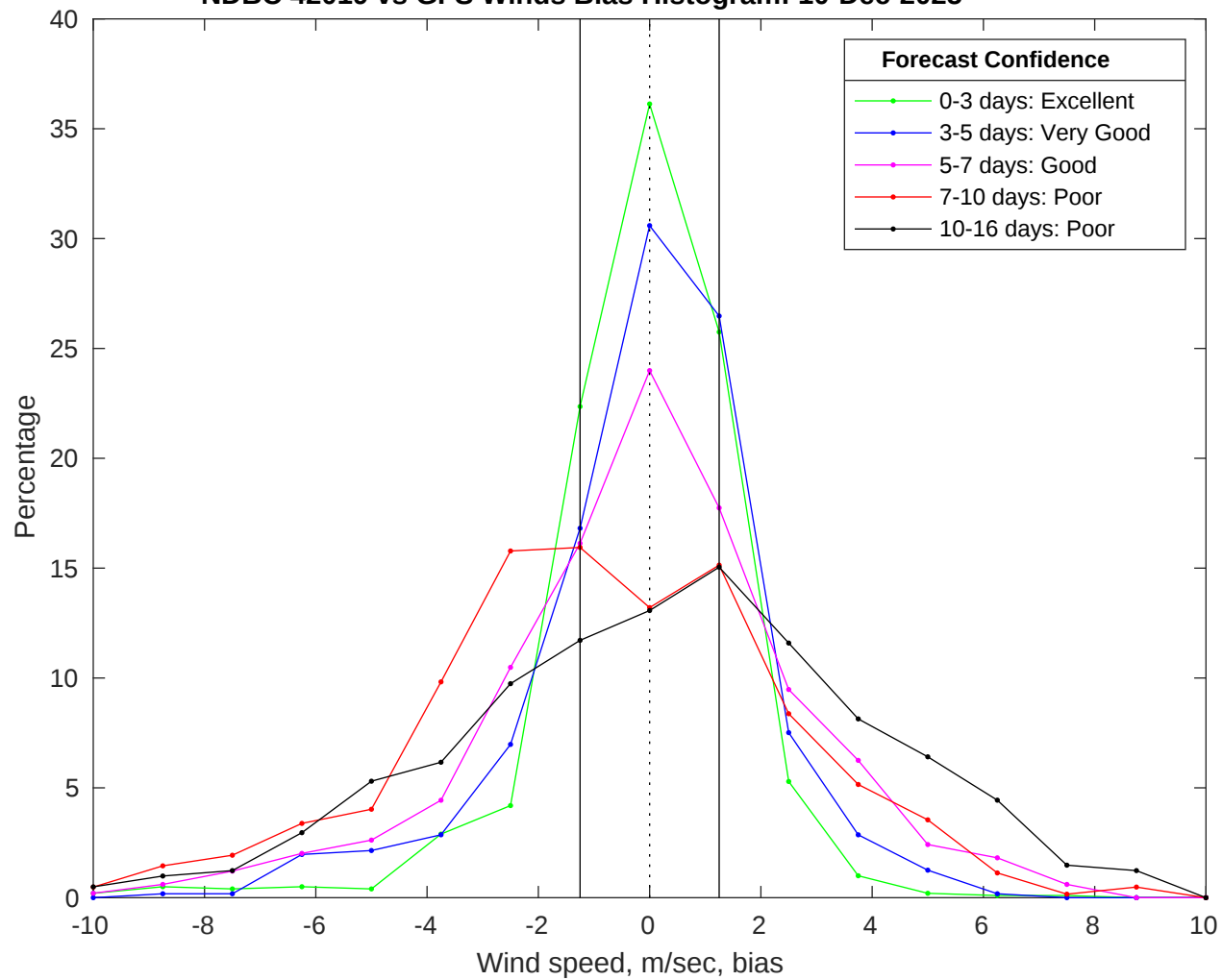
NDBC 42019 vs GFS Winds Bias Histogram: 10-Dec-2025
