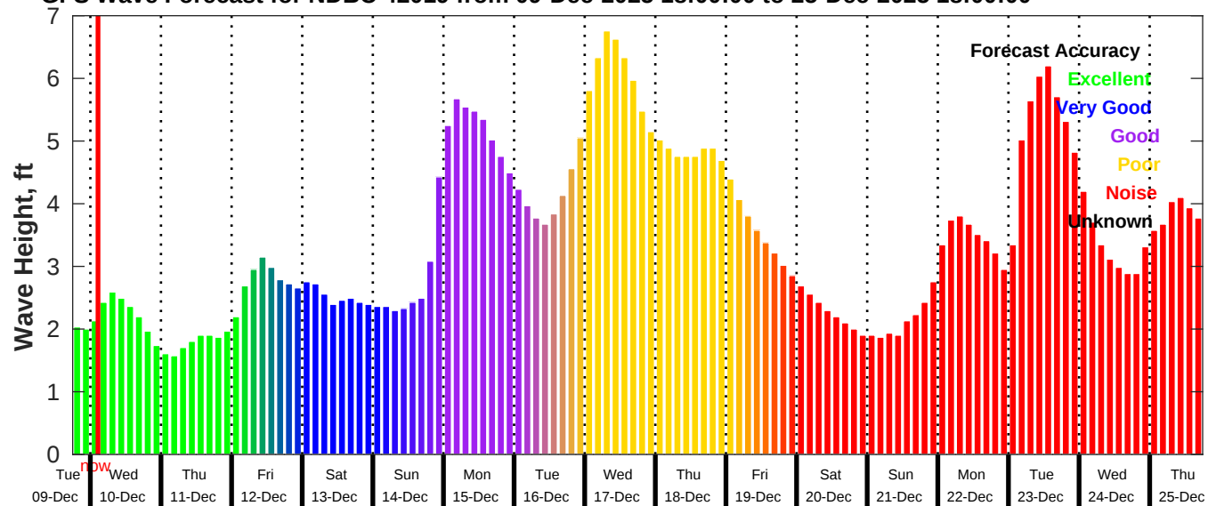
GFS Wave Forecast for NDBC 42019 from 09-Dec-2025 18:00:00 to 25-Dec-2025 18:00:00
