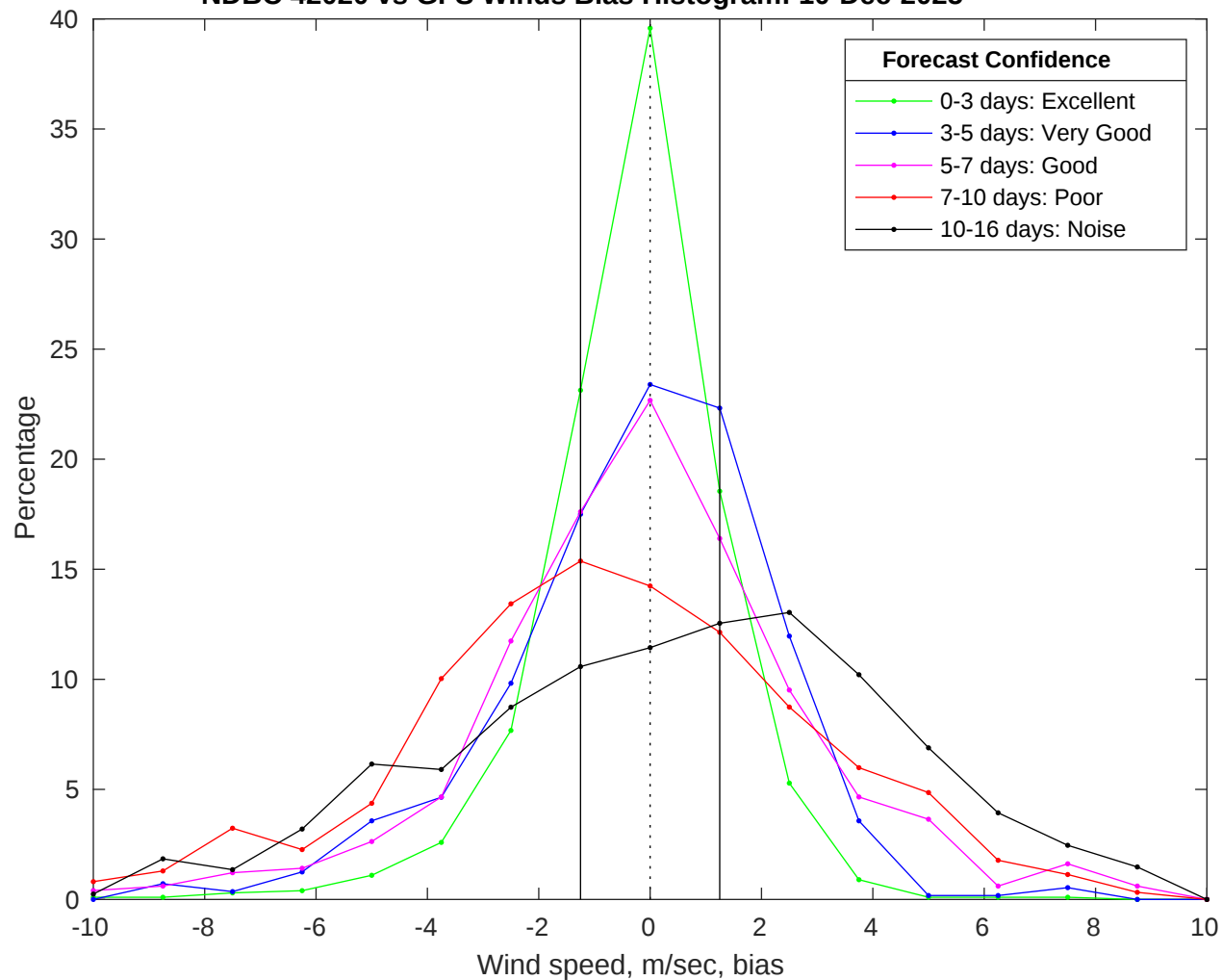
NDBC 42020 vs GFS Winds Bias Histogram: 10-Dec-2025
