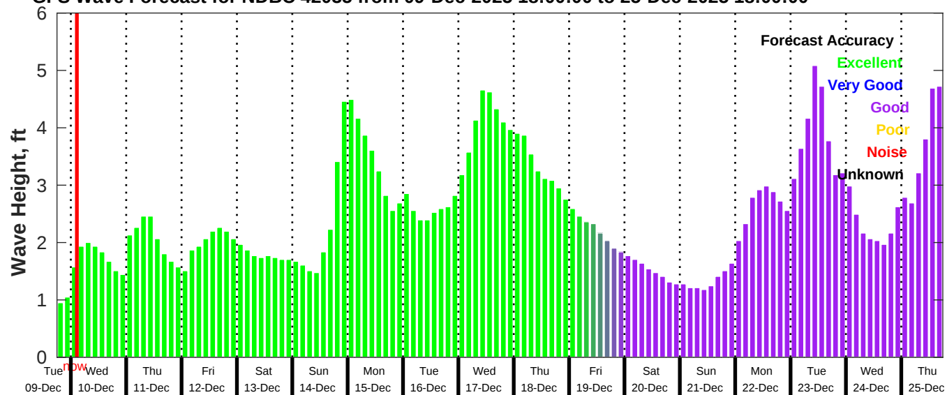
GFS Wave Forecast for NDBC 42035 from 09-Dec-2025 18:00:00 to 25-Dec-2025 18:00:00
