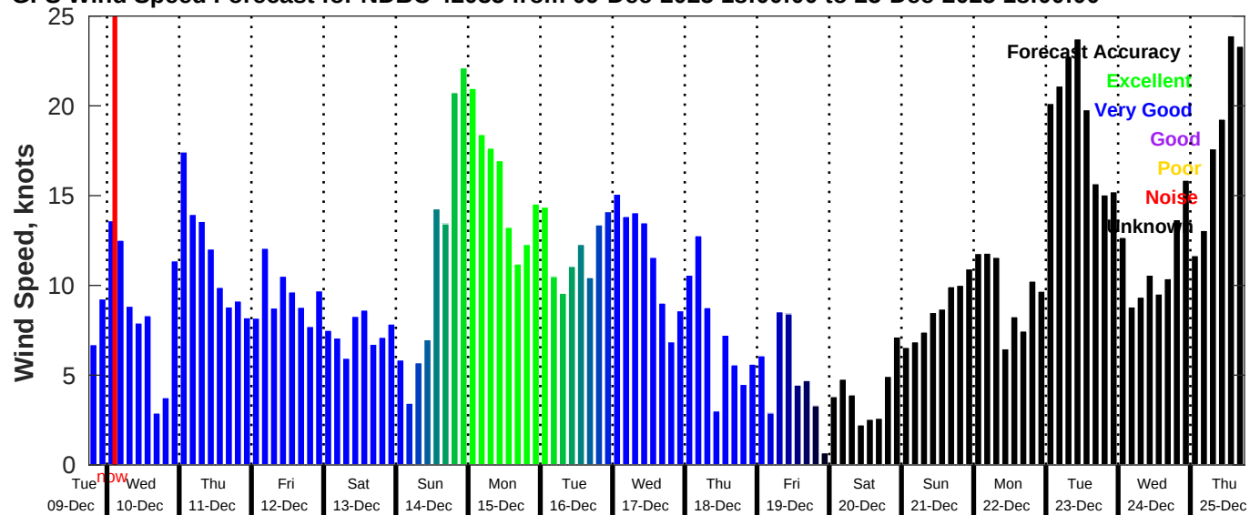
GFS Wind Speed Forecast for NDBC 42035 from 09-Dec-2025 18:00:00 to 25-Dec-2025 18:00:00
