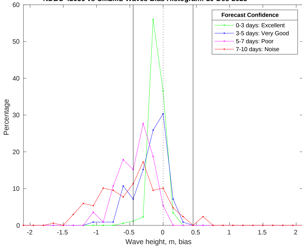
NDBC 42036 vs CMEMS Waves Bias Histogram: 10-Dec-2025
