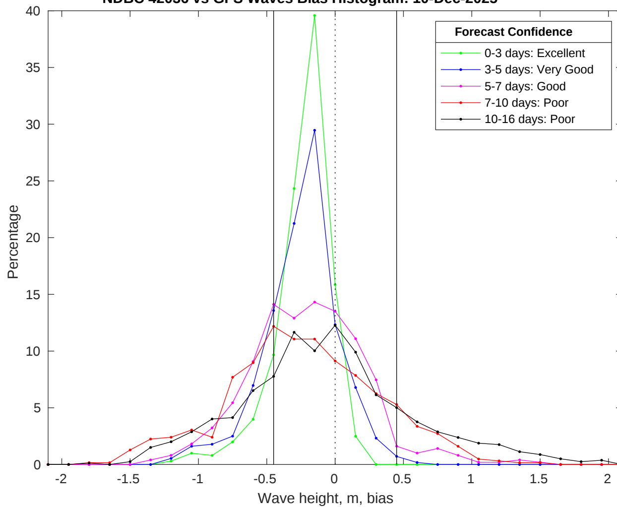
NDBC 42036 vs GFS Waves Bias Histogram: 10-Dec-2025
