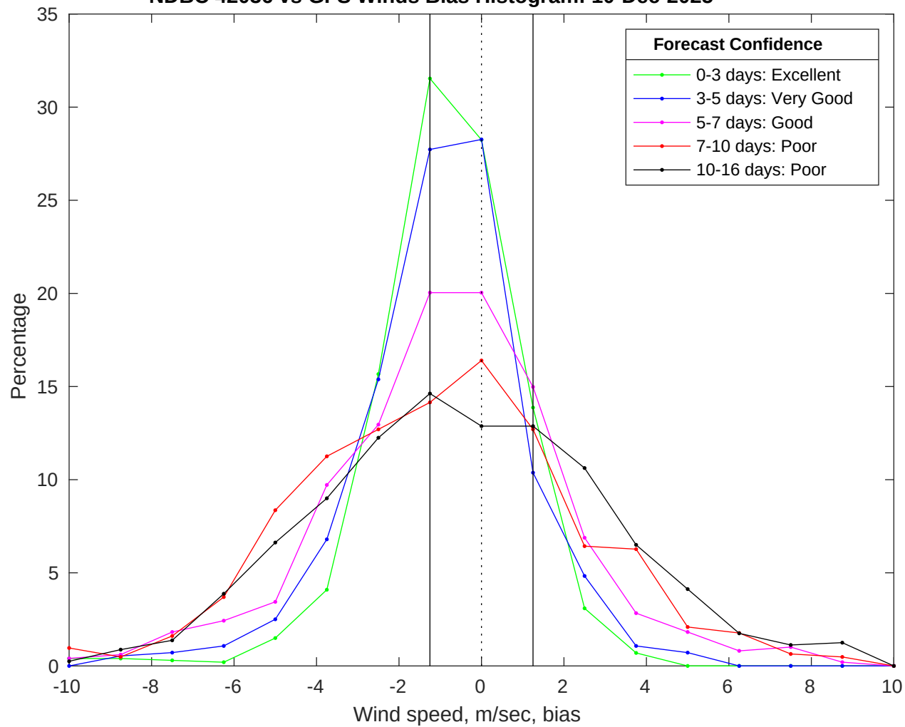
NDBC 42036 vs GFS Winds Bias Histogram: 10-Dec-2025
