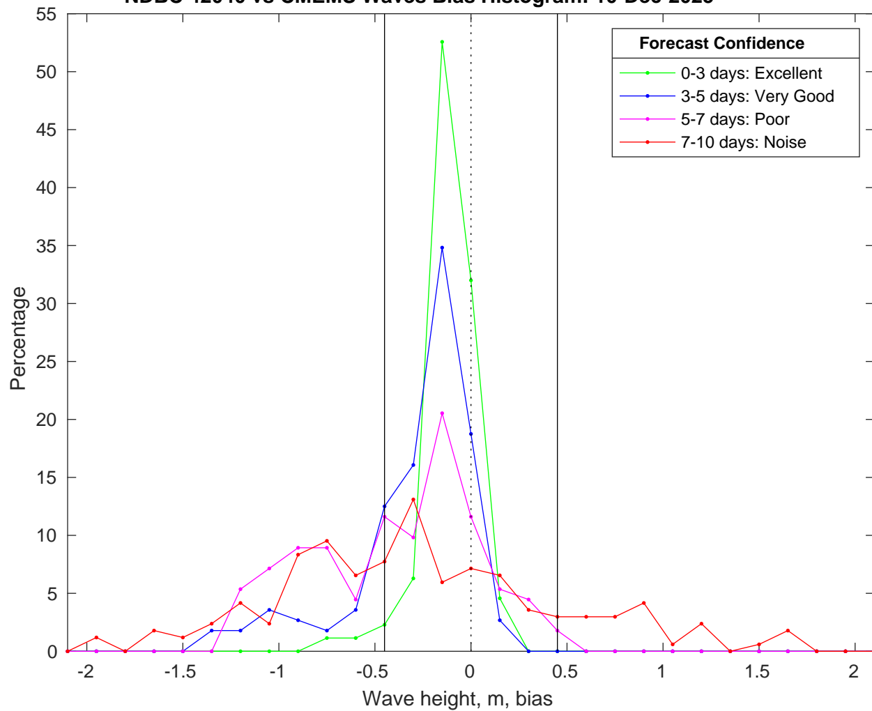
NDBC 42040 vs CMEMS Waves Bias Histogram: 10-Dec-2025
