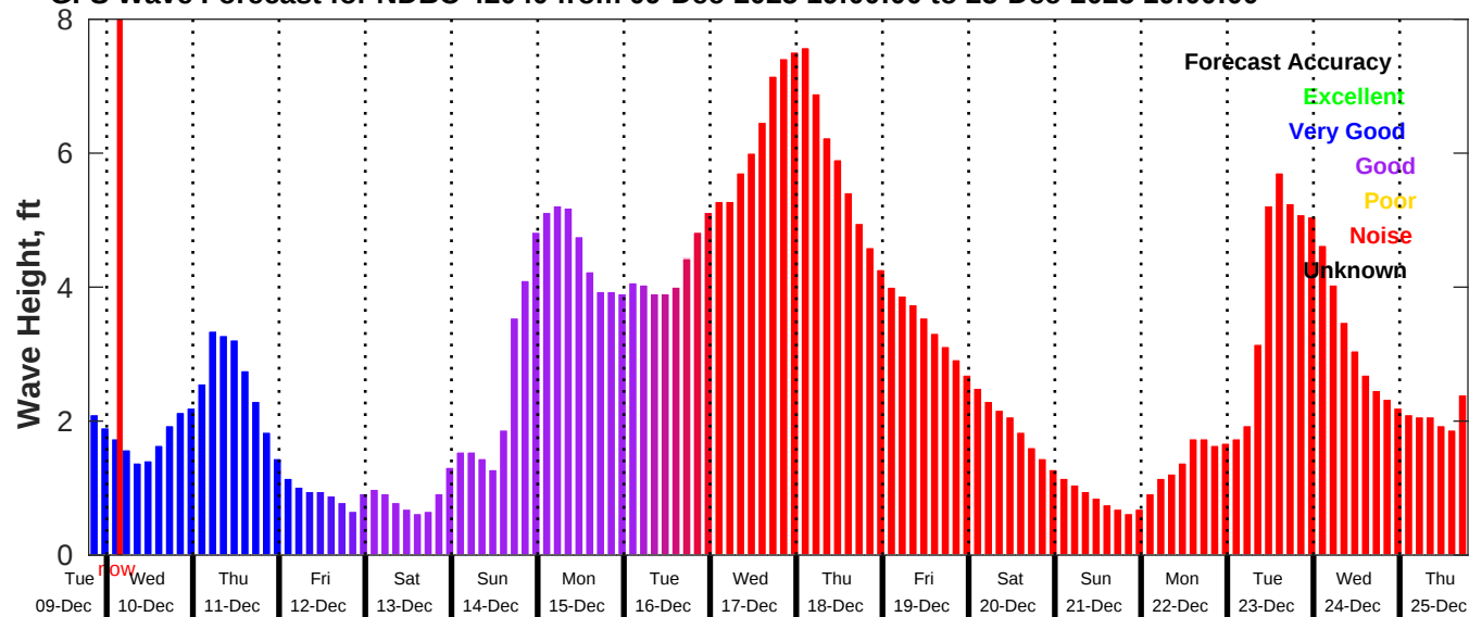
GFS Wave Forecast for NDBC 42040 from 09-Dec-2025 19:00:00 to 25-Dec-2025 19:00:00
