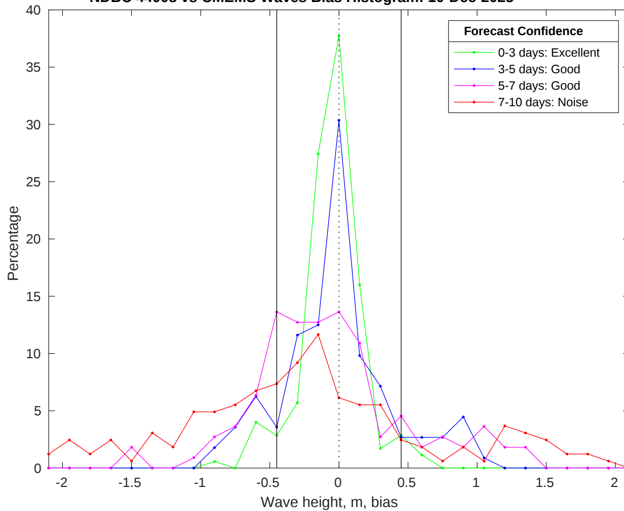
NDBC 44008 vs CMEMS Waves Bias Histogram: 10-Dec-2025
