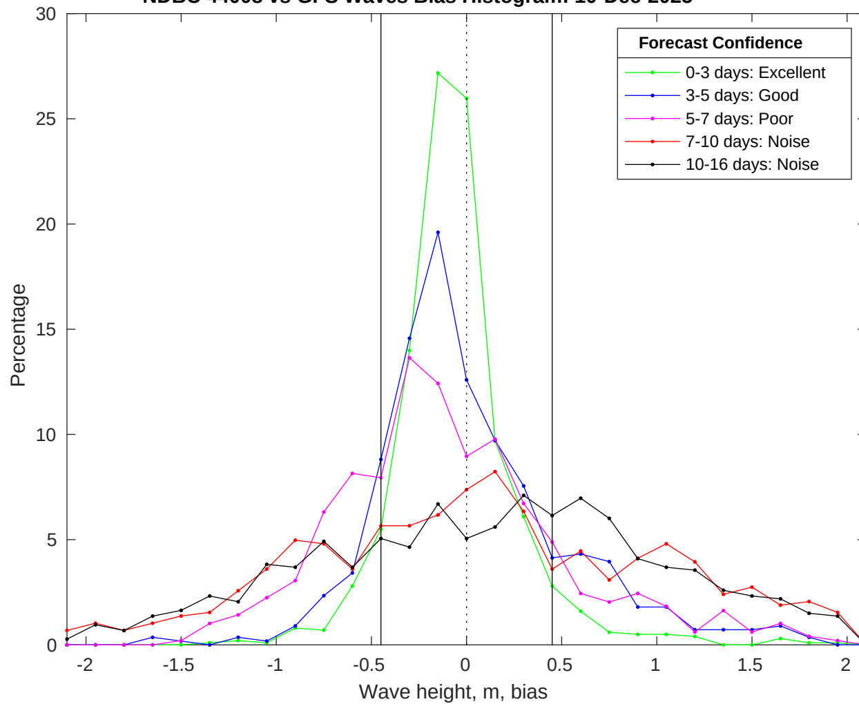
NDBC 44008 vs GFS Waves Bias Histogram: 10-Dec-2025
