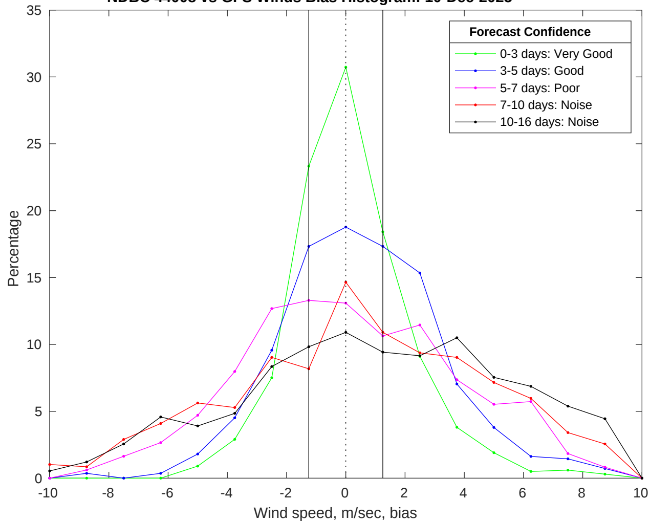
NDBC 44008 vs GFS Winds Bias Histogram: 10-Dec-2025
