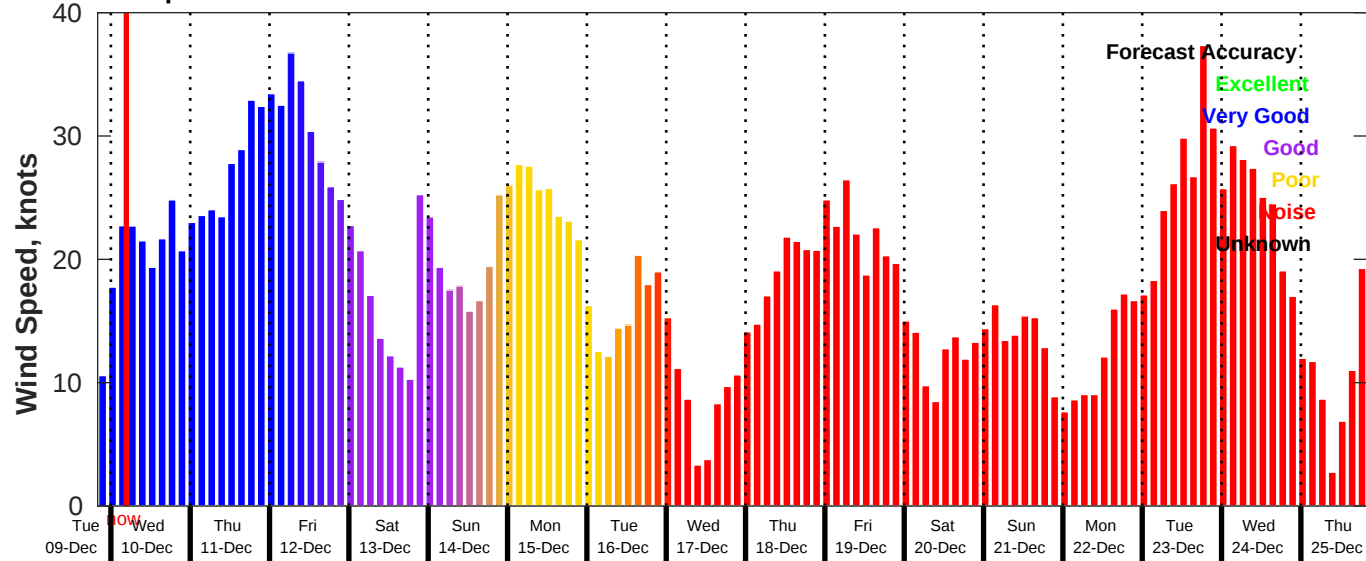
GFS Wind Speed Forecast for NDBC 44008 from 09-Dec-2025 20:00:00 to 25-Dec-2025 20:00:00
