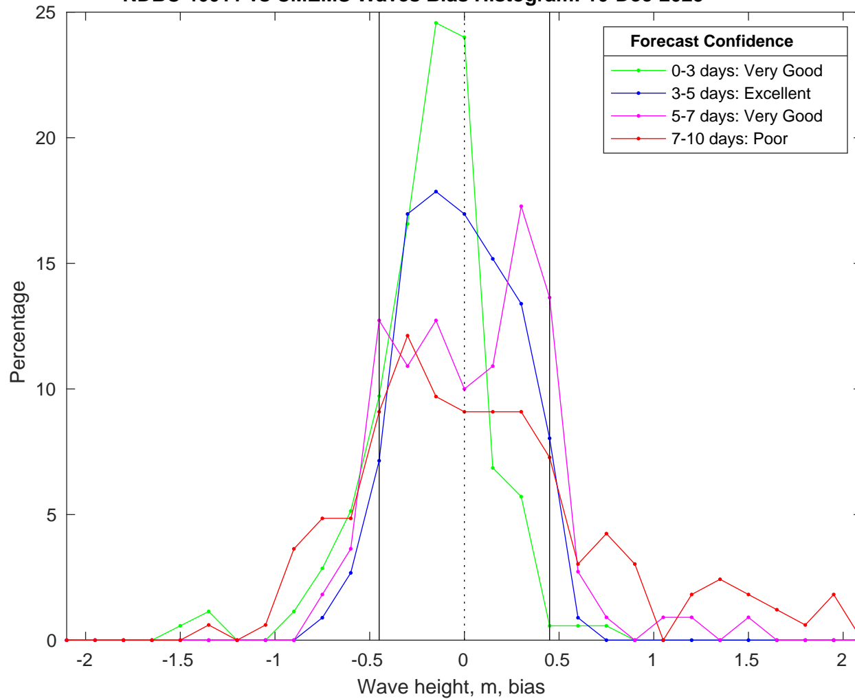
NDBC 46011 vs CMEMS Waves Bias Histogram: 10-Dec-2025
