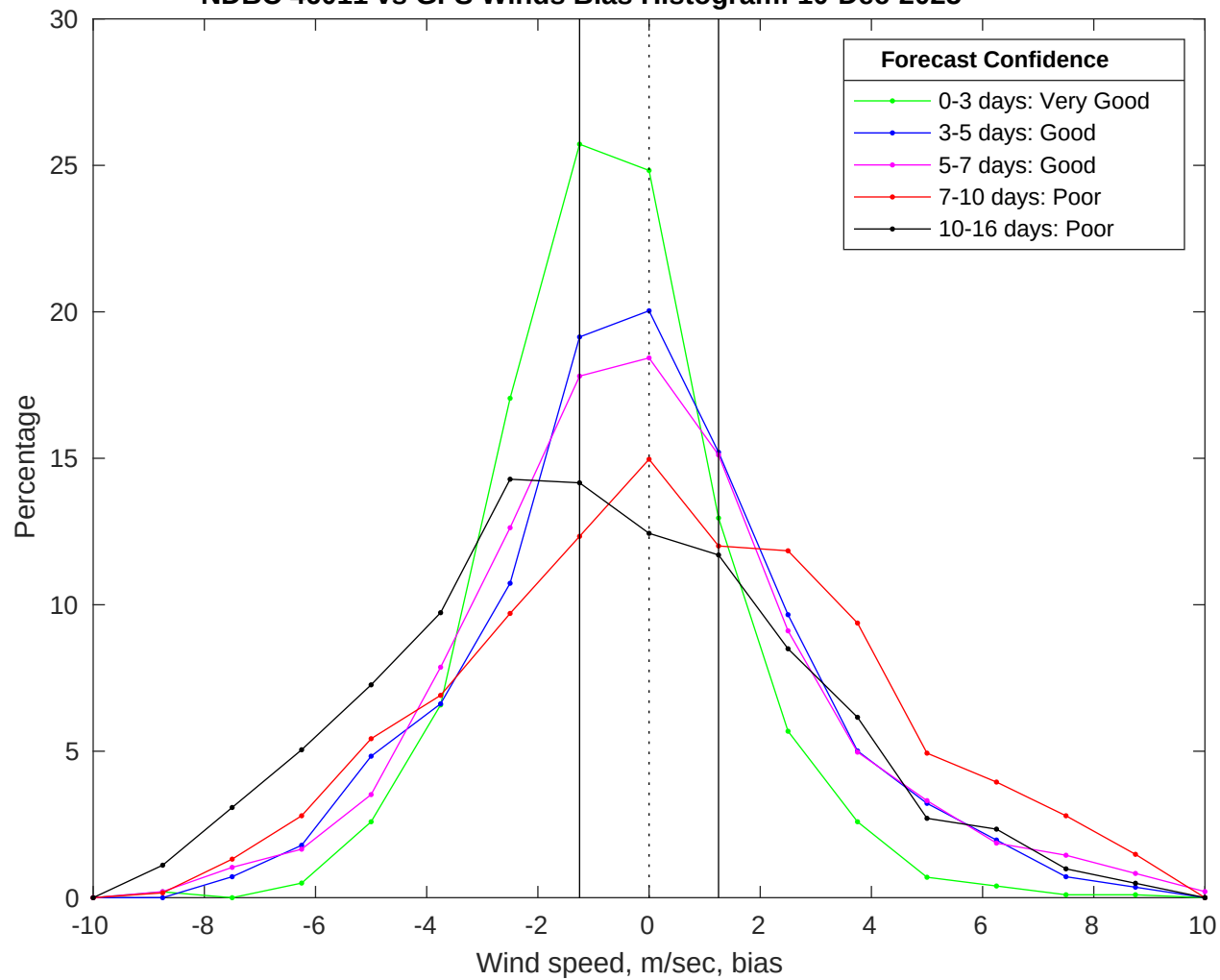
NDBC 46011 vs GFS Winds Bias Histogram: 10-Dec-2025
