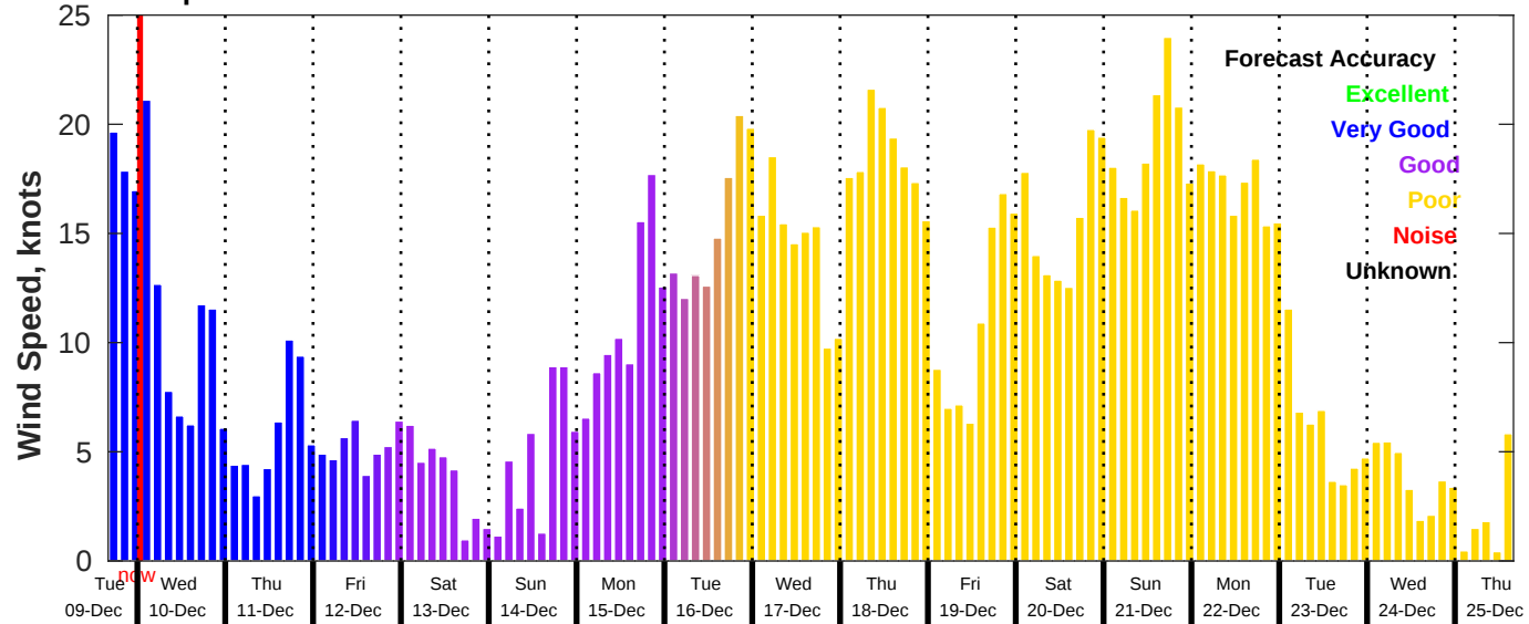
GFS Wind Speed Forecast for NDBC 46011 from 09-Dec-2025 16:00:00 to 25-Dec-2025 16:00:00
