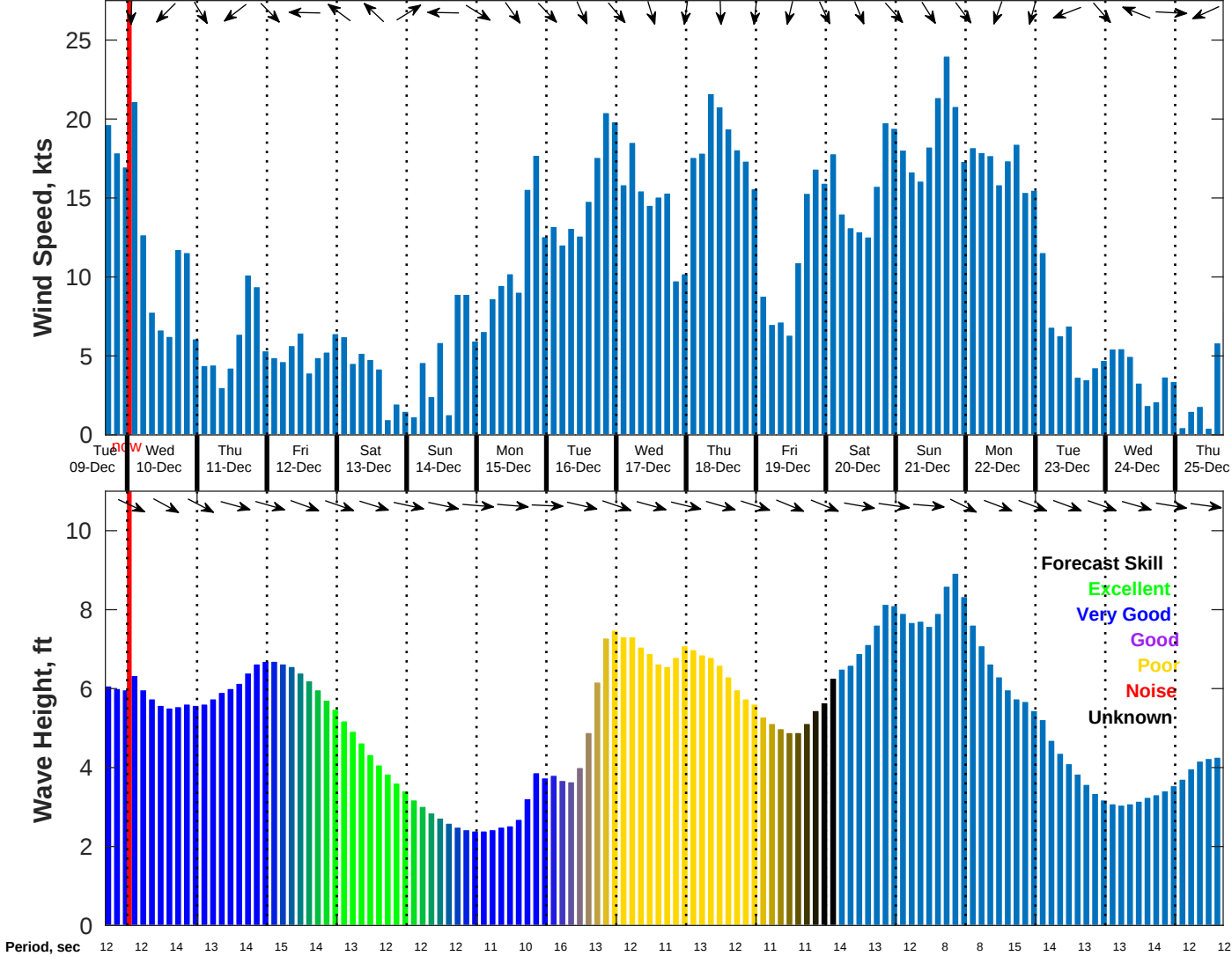
Wind & Wave Forecast for NDBC 46011 from 09-Dec-2025 16:00:00 to 25-Dec-2025 16:00:00
