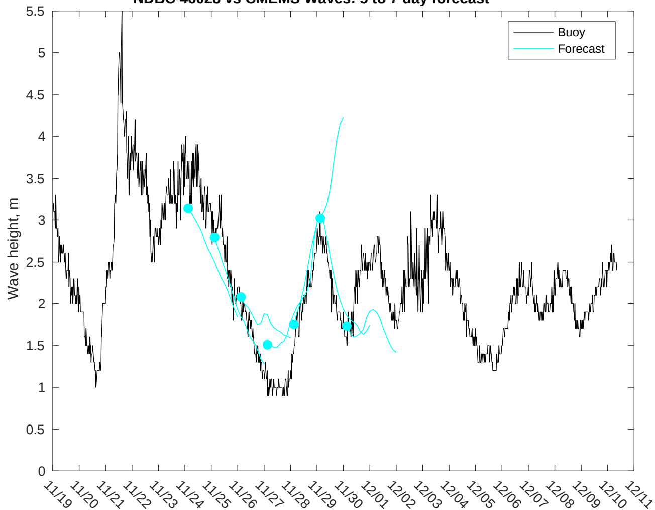
NDBC 46028 vs CMEMS Waves: 5 to 7 day forecast
