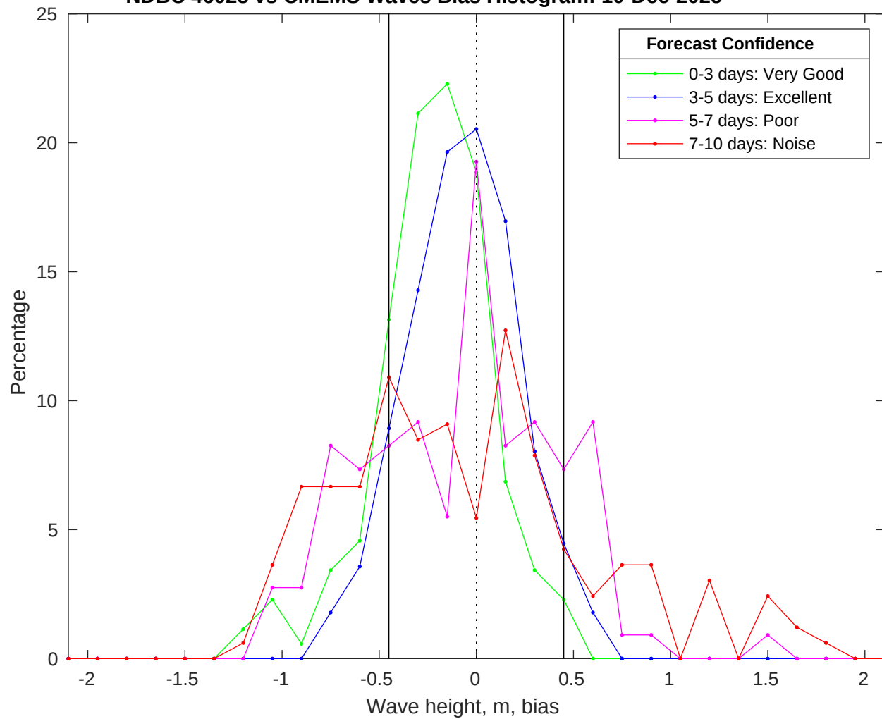
NDBC 46028 vs CMEMS Waves Bias Histogram: 10-Dec-2025
