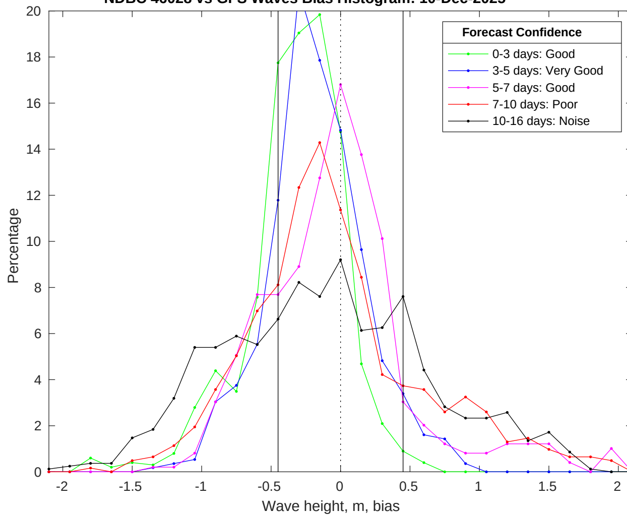
NDBC 46028 vs GFS Waves Bias Histogram: 10-Dec-2025
