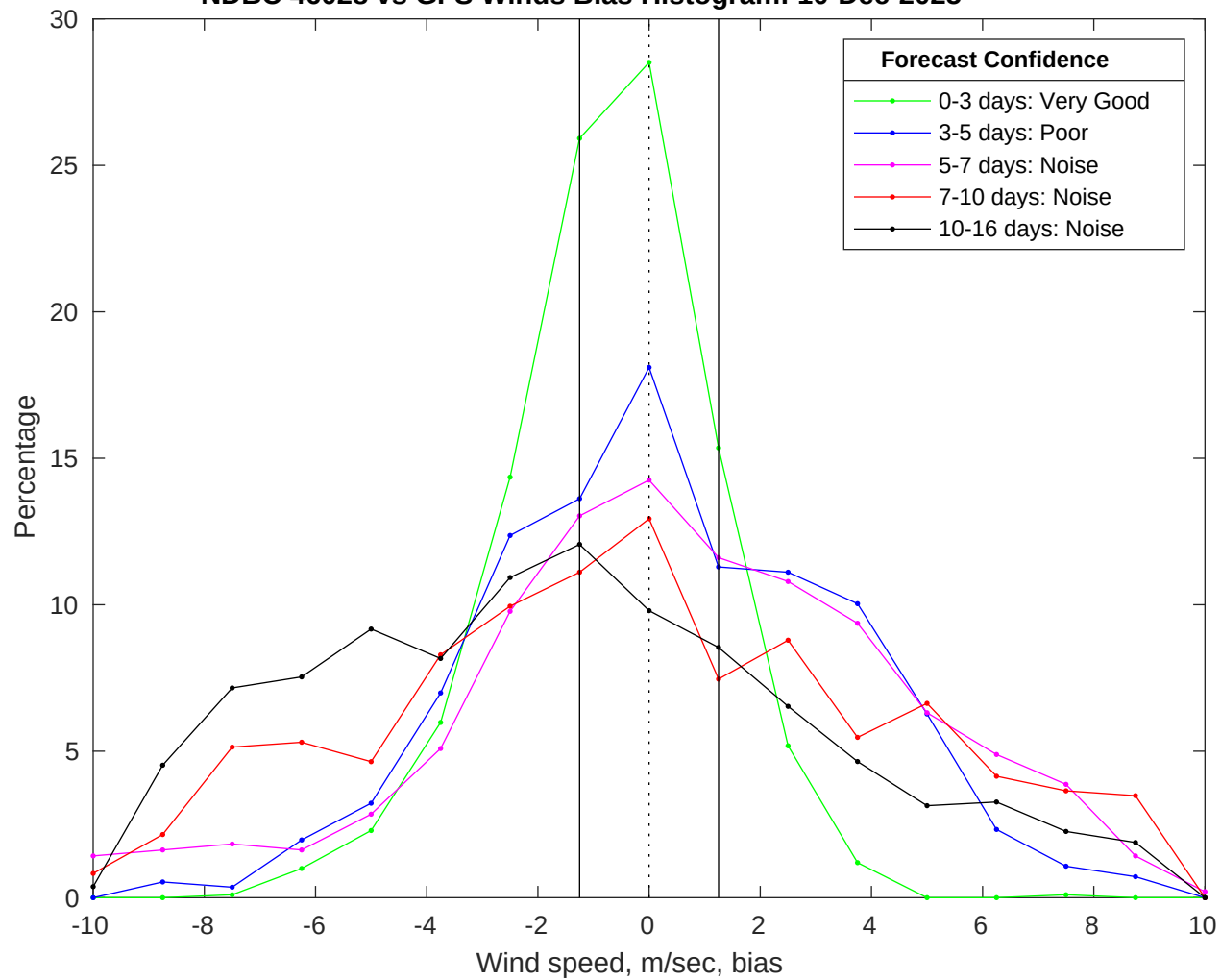
NDBC 46028 vs GFS Winds Bias Histogram: 10-Dec-2025
