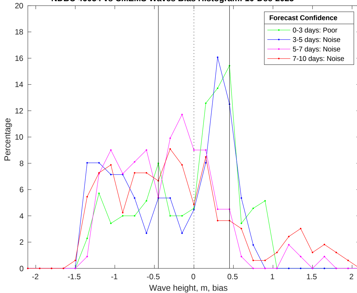
NDBC 46054 vs CMEMS Waves Bias Histogram: 10-Dec-2025
