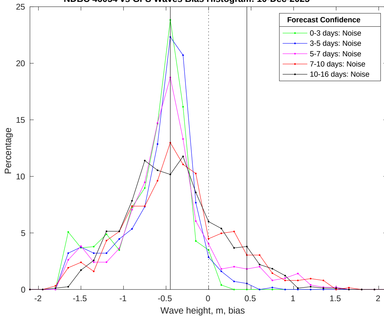
NDBC 46054 vs GFS Waves Bias Histogram: 10-Dec-2025
