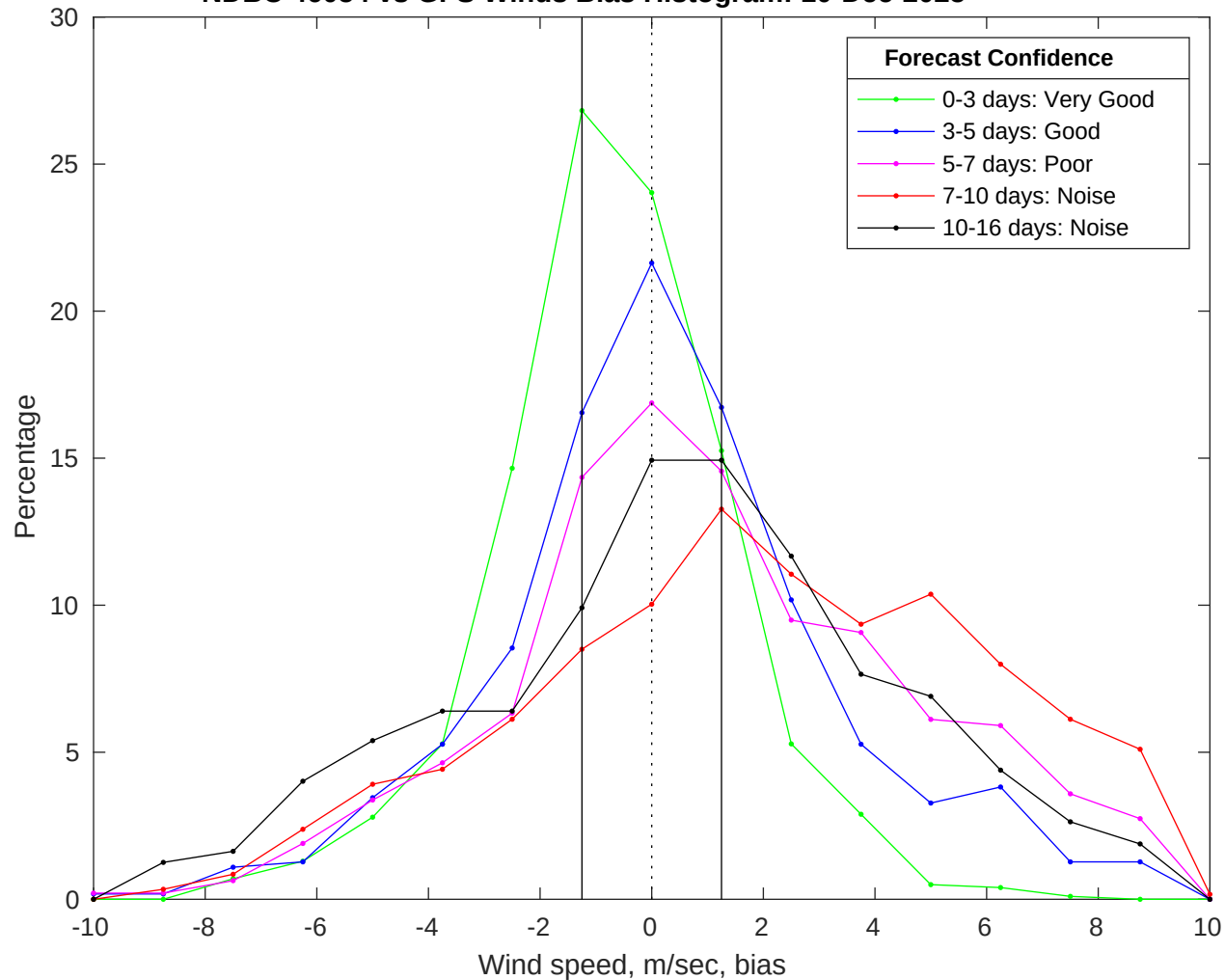
NDBC 46054 vs GFS Winds Bias Histogram: 10-Dec-2025
