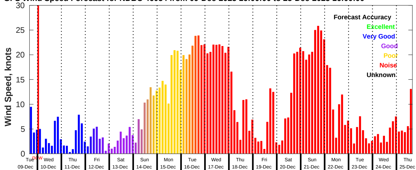
GFS Wind Speed Forecast for NDBC 46054 from 09-Dec-2025 16:00:00 to 25-Dec-2025 16:00:00
