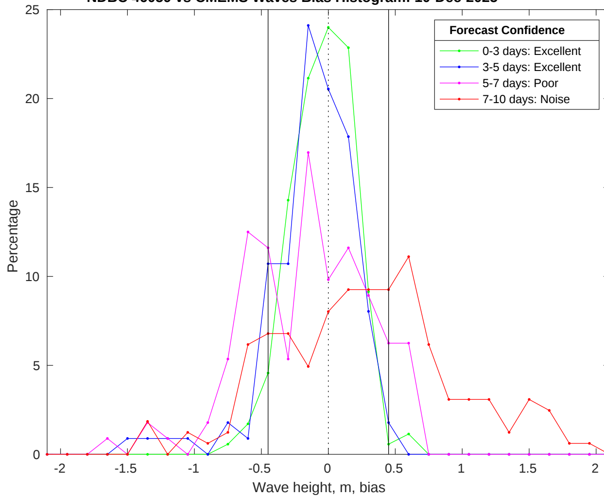
NDBC 46059 vs CMEMS Waves Bias Histogram: 10-Dec-2025
