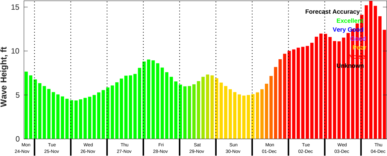
CMEMS Wave Forecast for NDBC 46059 from 24-Nov-2025 17:00:00 to 04-Dec-2025 17:00:00
