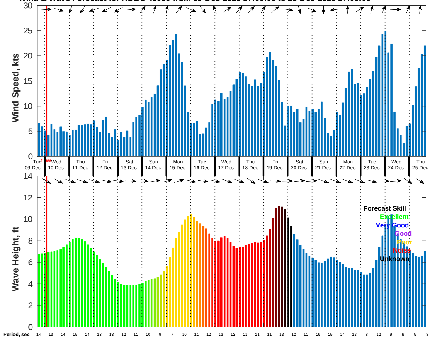
Wind & Wave Forecast for NDBC 46059 from 09-Dec-2025 17:00:00 to 25-Dec-2025 17:00:00
