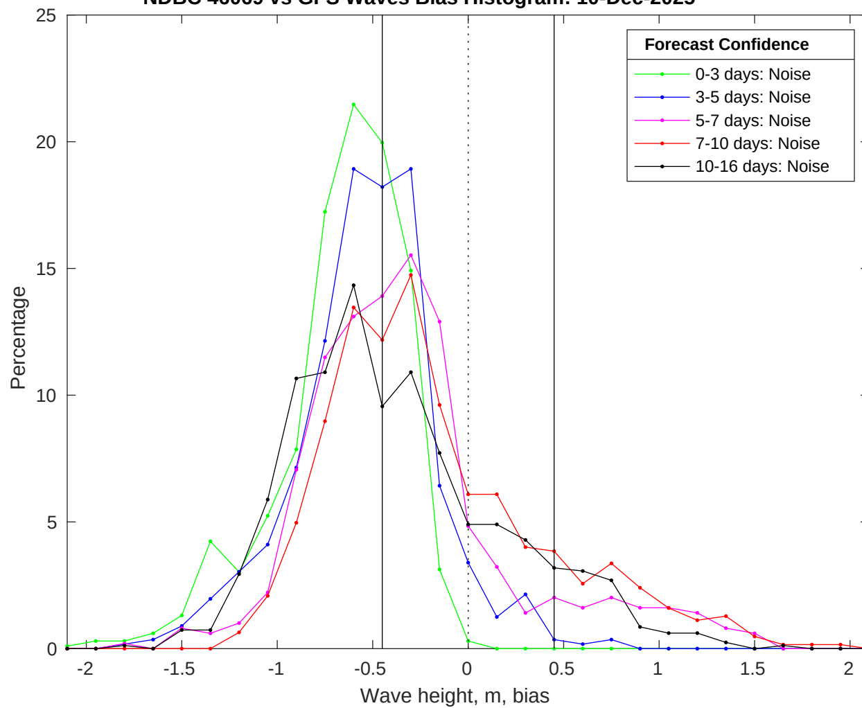
NDBC 46069 vs GFS Waves Bias Histogram: 10-Dec-2025
