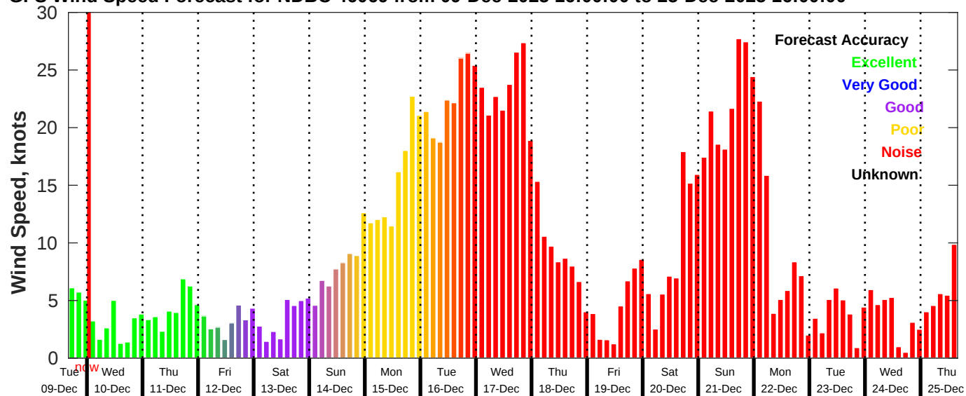
GFS Wind Speed Forecast for NDBC 46069 from 09-Dec-2025 16:00:00 to 25-Dec-2025 16:00:00
