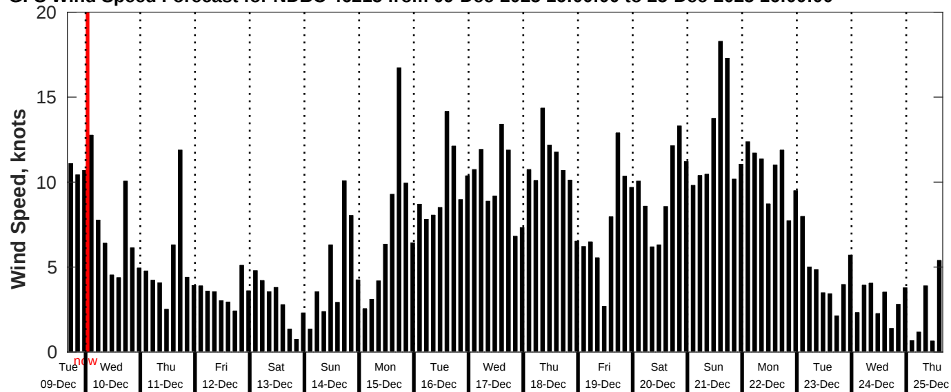
GFS Wind Speed Forecast for NDBC 46215 from 09-Dec-2025 16:00:00 to 25-Dec-2025 16:00:00
