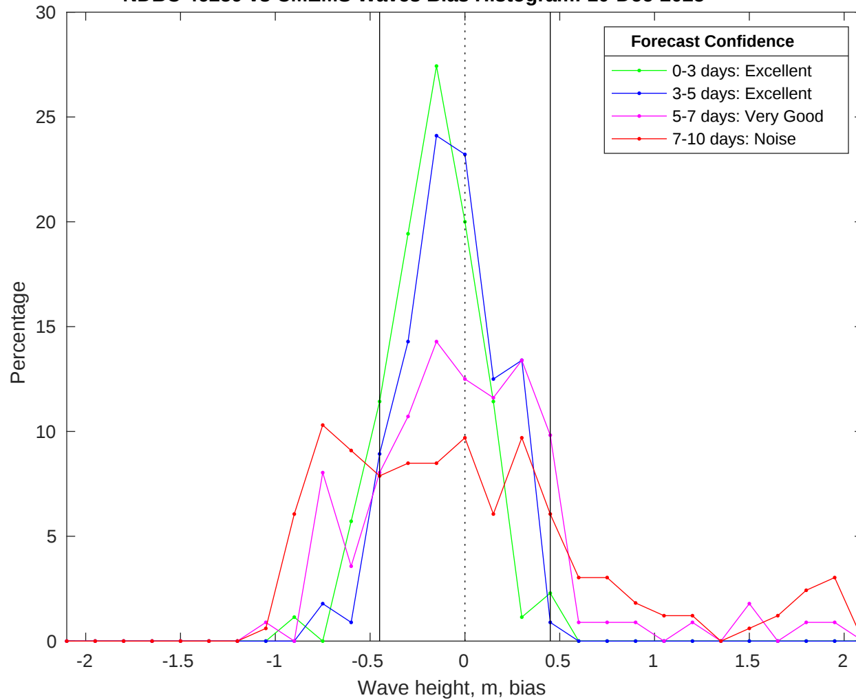
NDBC 46259 vs CMEMS Waves Bias Histogram: 10-Dec-2025
