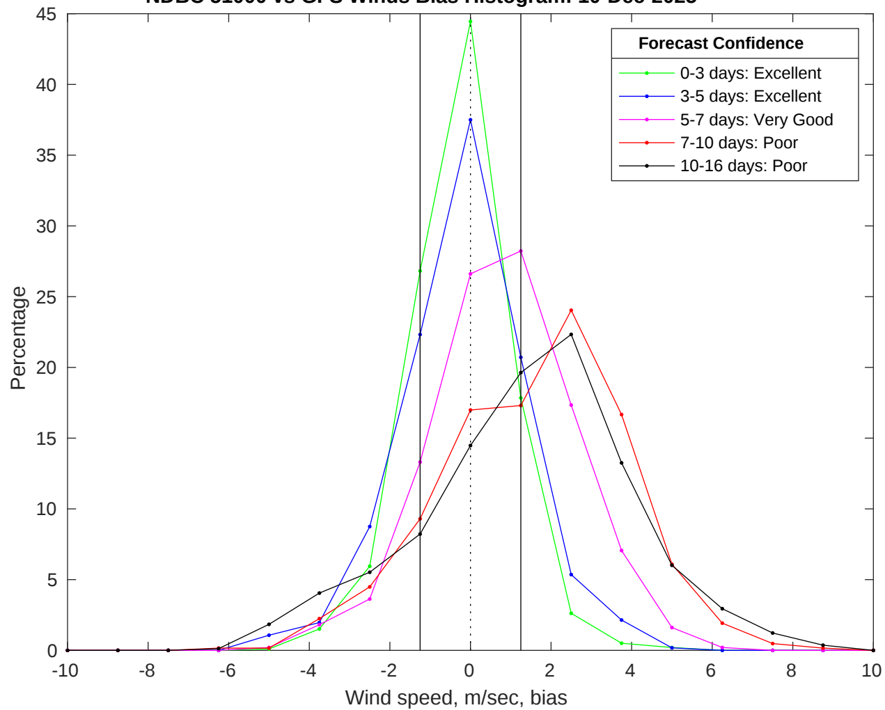
NDBC 51000 vs GFS Winds Bias Histogram: 10-Dec-2025
