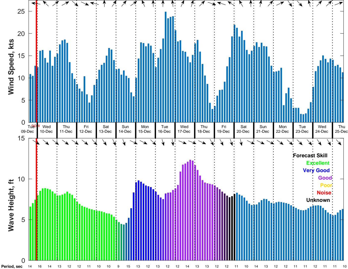
Wind & Wave Forecast for NDBC 51000 from 09-Dec-2025 14:00:00 to 25-Dec-2025 14:00:00
