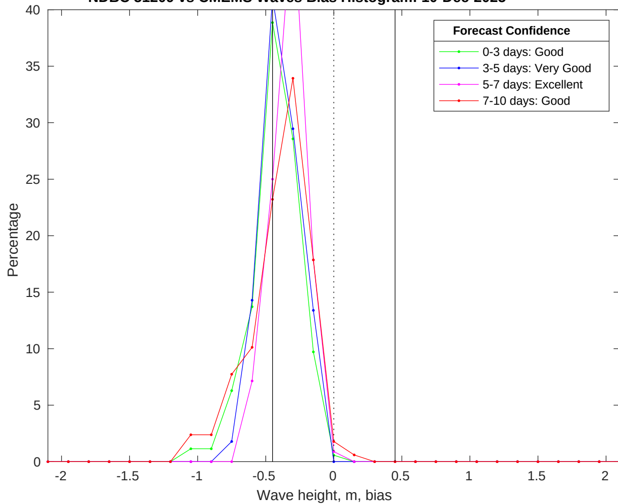
NDBC 51209 vs CMEMS Waves Bias Histogram: 10-Dec-2025
