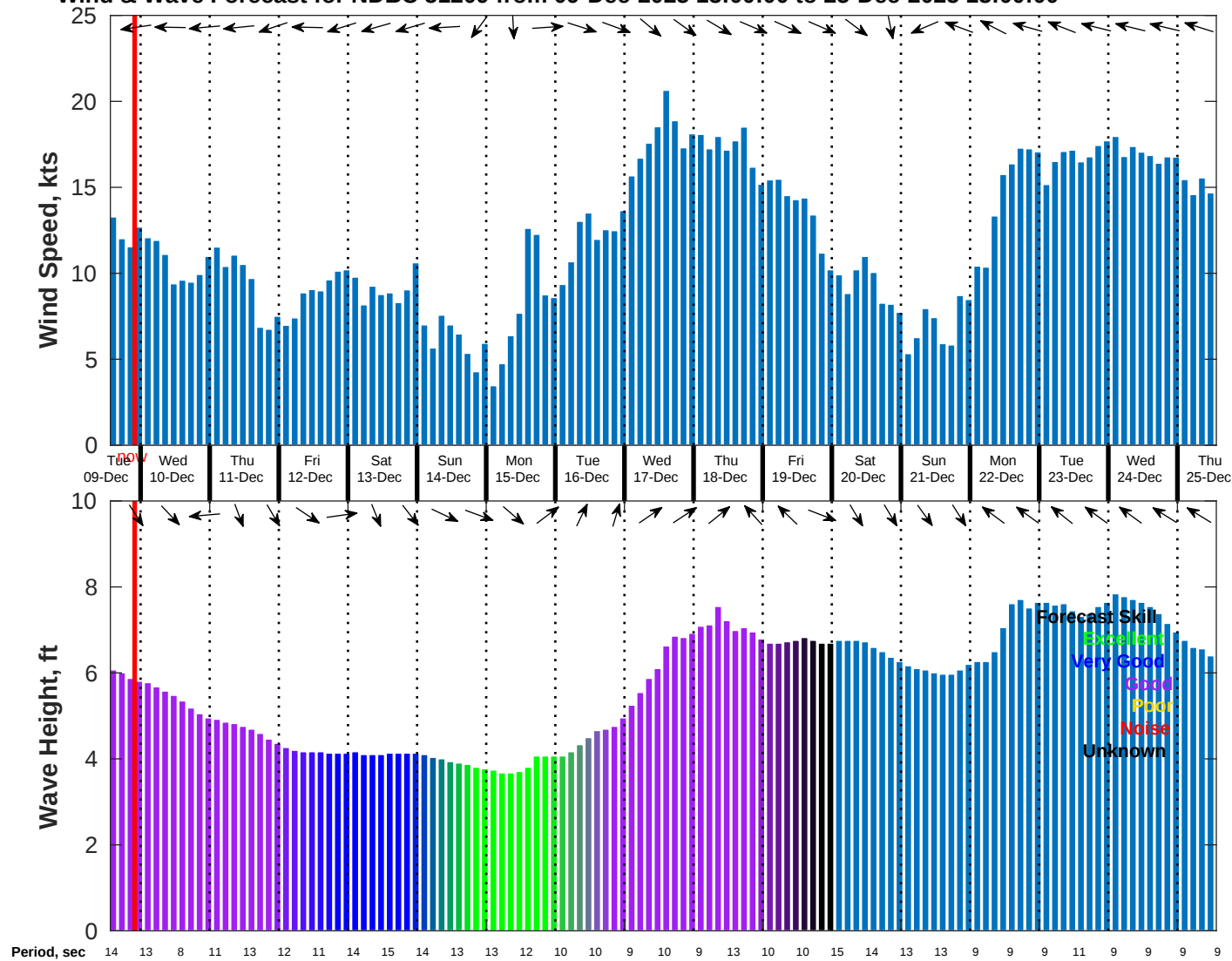
Wind & Wave Forecast for NDBC 51209 from 09-Dec-2025 13:00:00 to 25-Dec-2025 13:00:00
