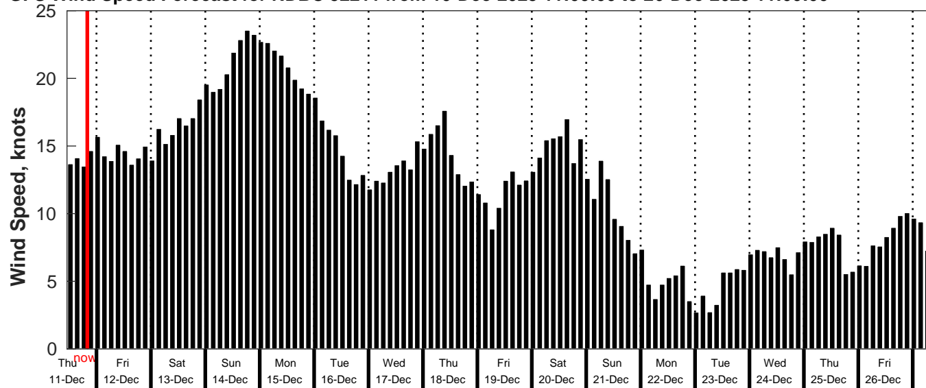
GFS Wind Speed Forecast for NDBC 52211 from 10-Dec-2025 11:00:00 to 26-Dec-2025 11:00:00
