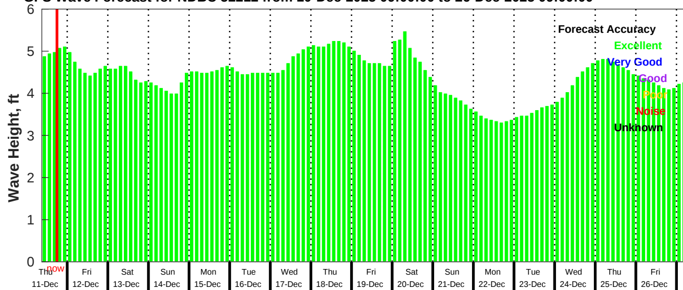
GFS Wave Forecast for NDBC 52212 from 10-Dec-2025 09:00:00 to 26-Dec-2025 09:00:00
