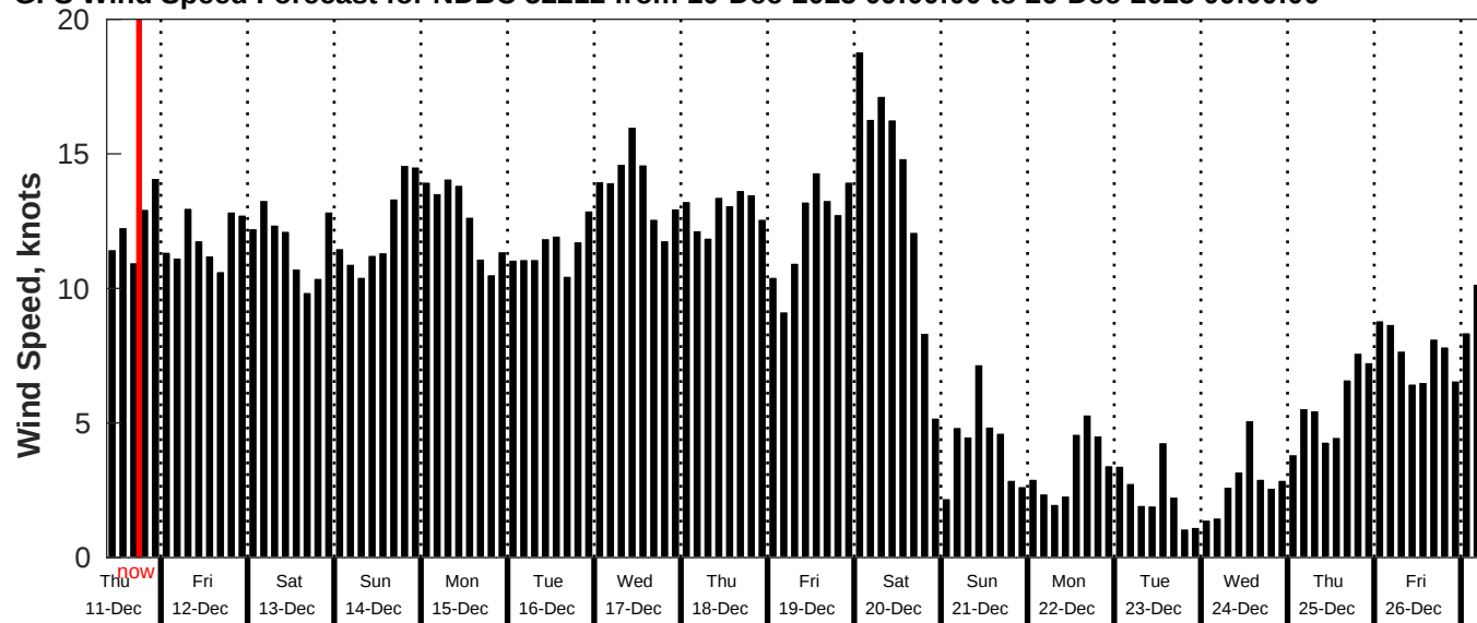
GFS Wind Speed Forecast for NDBC 52212 from 10-Dec-2025 09:00:00 to 26-Dec-2025 09:00:00
