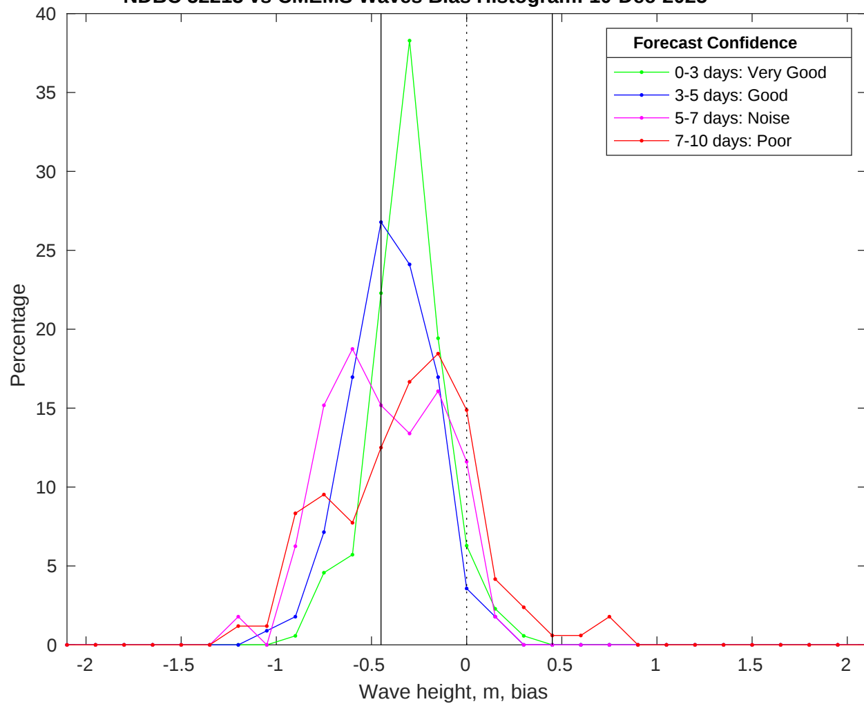
NDBC 52213 vs CMEMS Waves Bias Histogram: 10-Dec-2025
