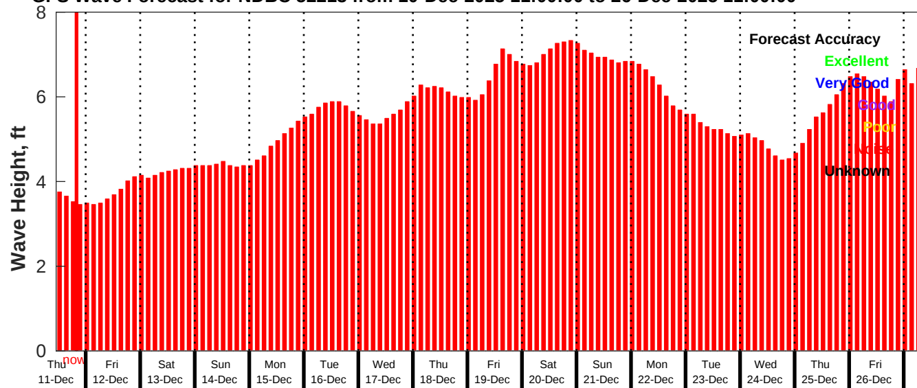
GFS Wave Forecast for NDBC 52213 from 10-Dec-2025 11:00:00 to 26-Dec-2025 11:00:00
